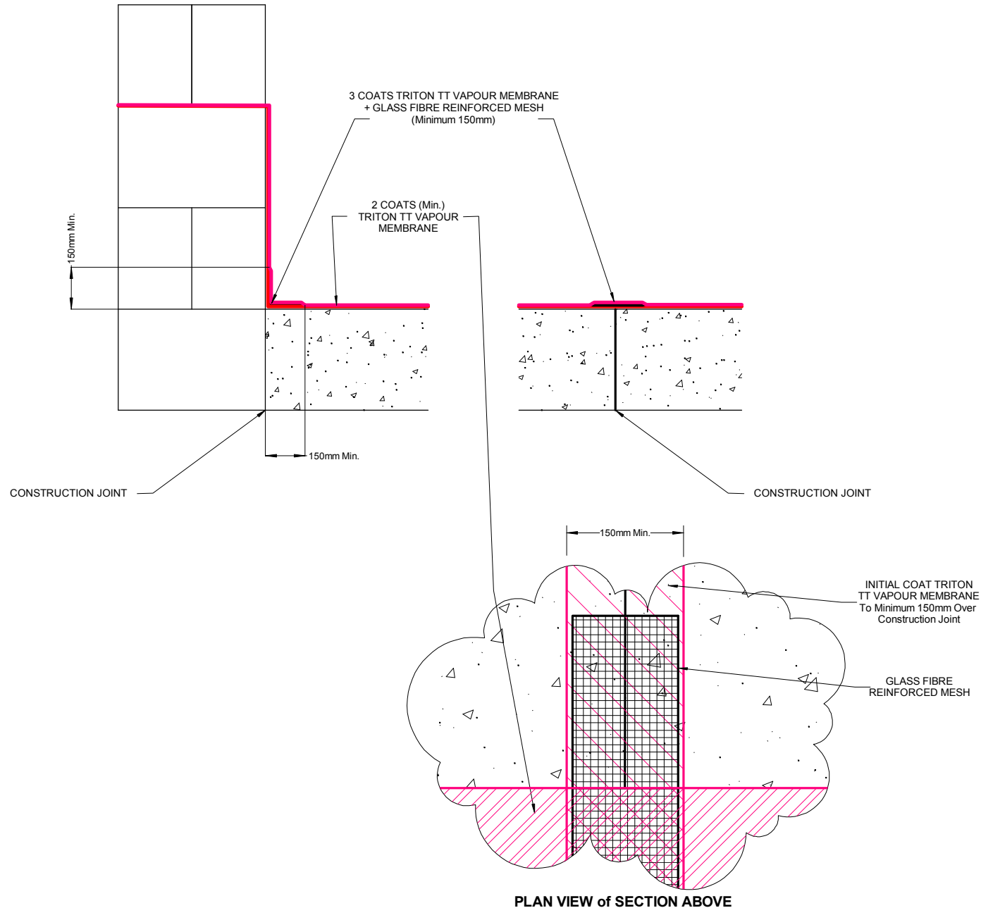
PLAN VIEW of SECTION ABOVE
